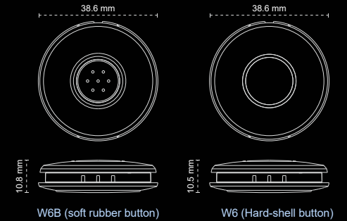
W6B (soft rubber button)
