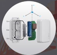
Built-in accelerometer
