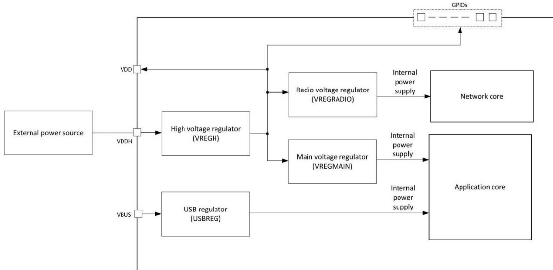
Figure 7: Regulator usage in high voltage mode
