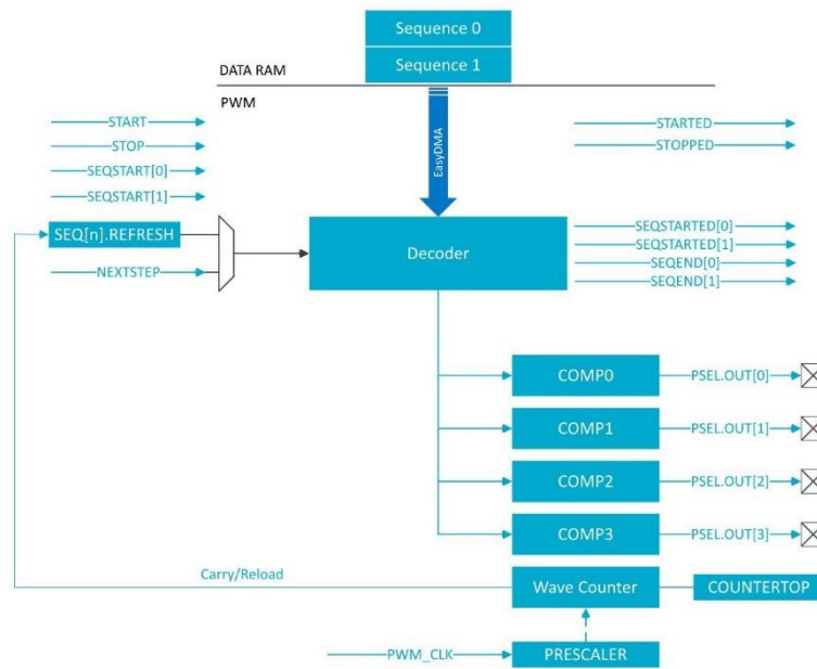
Figure 10: PWM module
