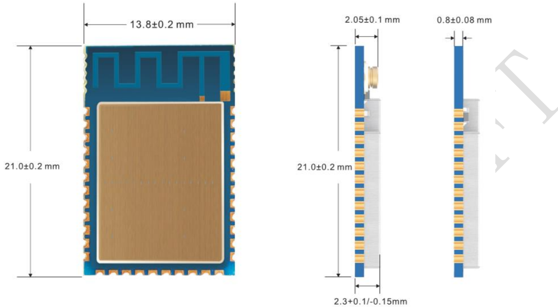
Figure 3: MK13 PCBA dimensions
