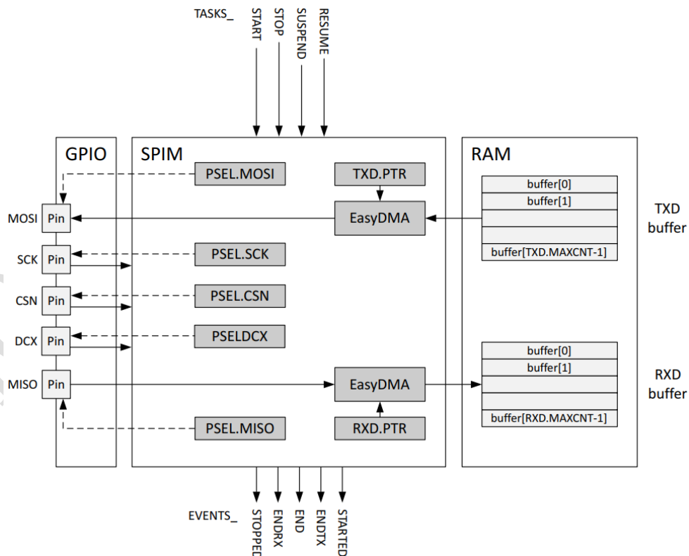
Figure 12: SPIM with EasyDMA
