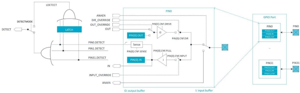
Figure 11: GPIO port and the GPIO pin details
