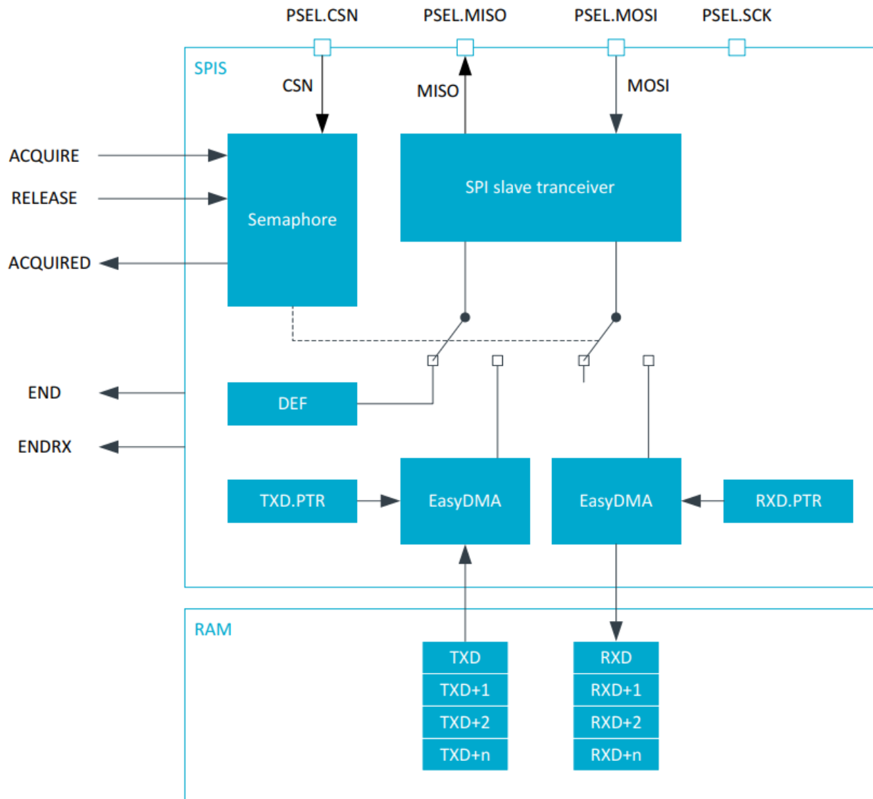
Figure 13: SPI slave
