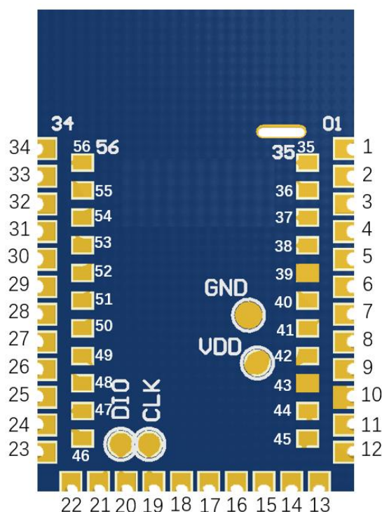
Figure 2: MK13 pin diagram (Rear View)
