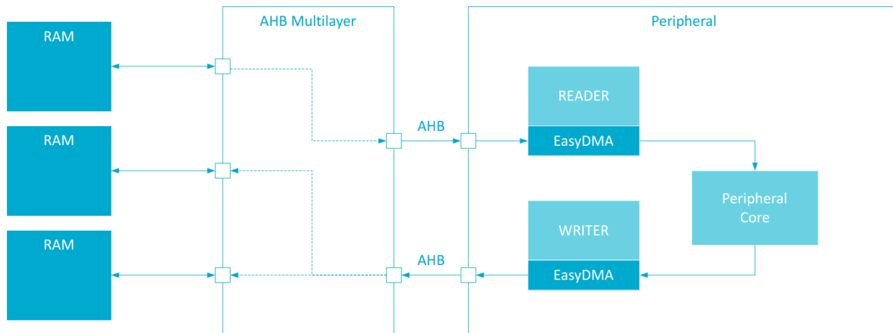
Figure 17: EasyDMA example
