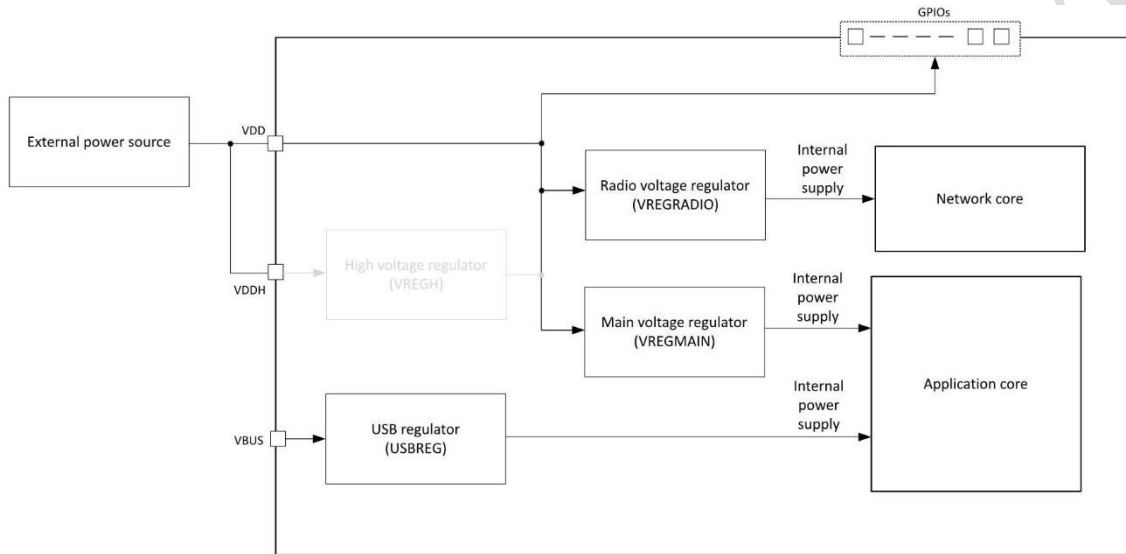
Figure 6: Regulator usage in normal voltage mode
