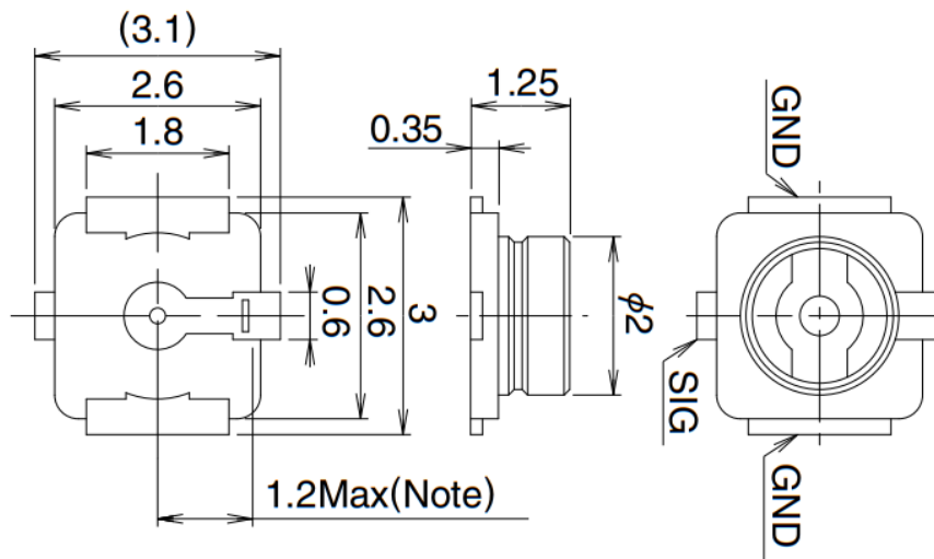
Figure 5: u.FL-R-SMT-1(80) Dimensions
