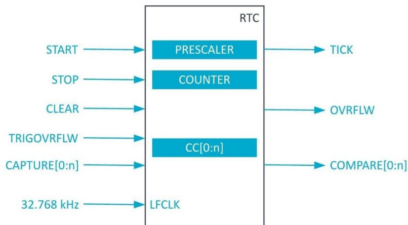
Figure 9: RTC Block Diagram
