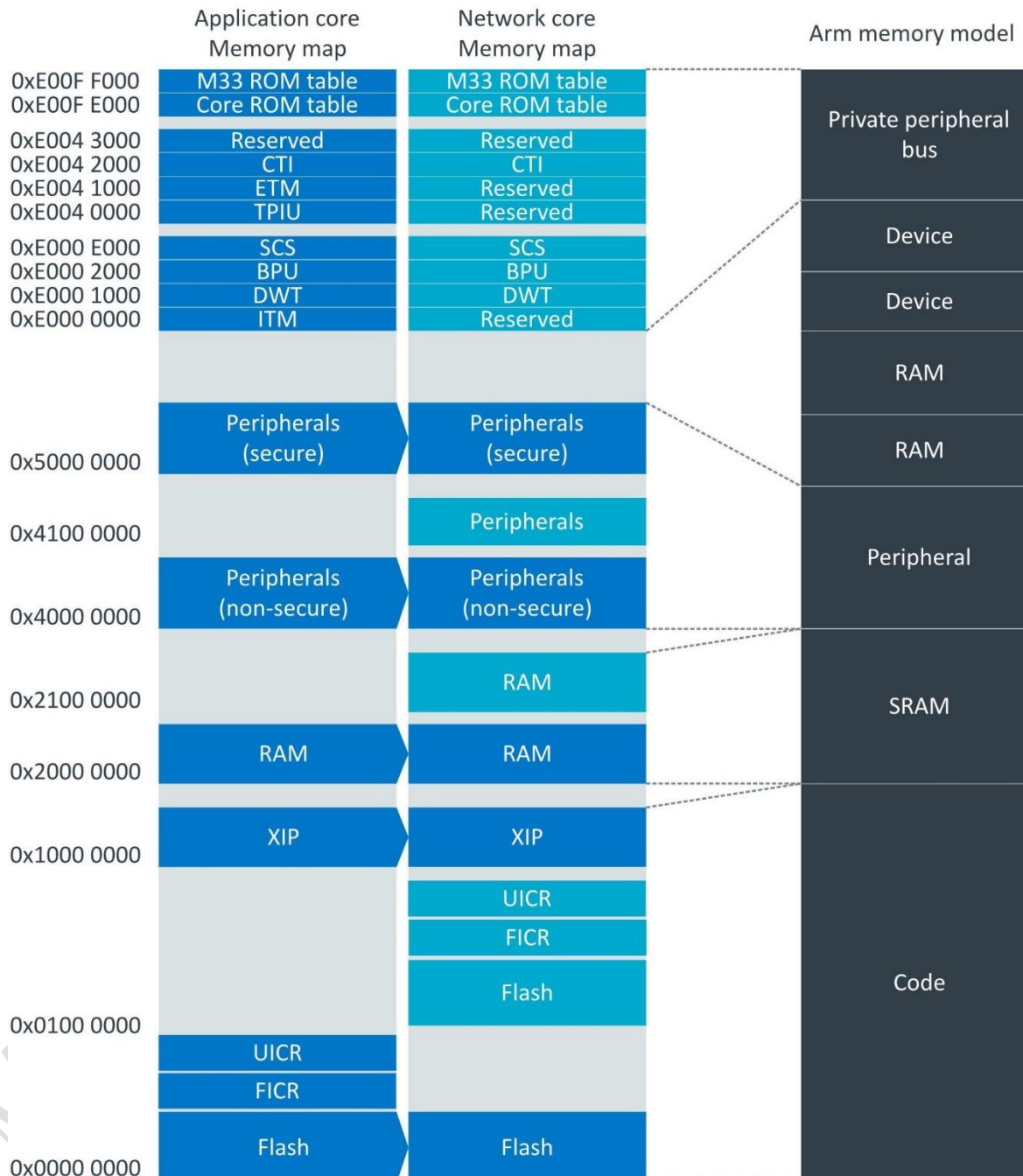
Figure 8: Memory map
