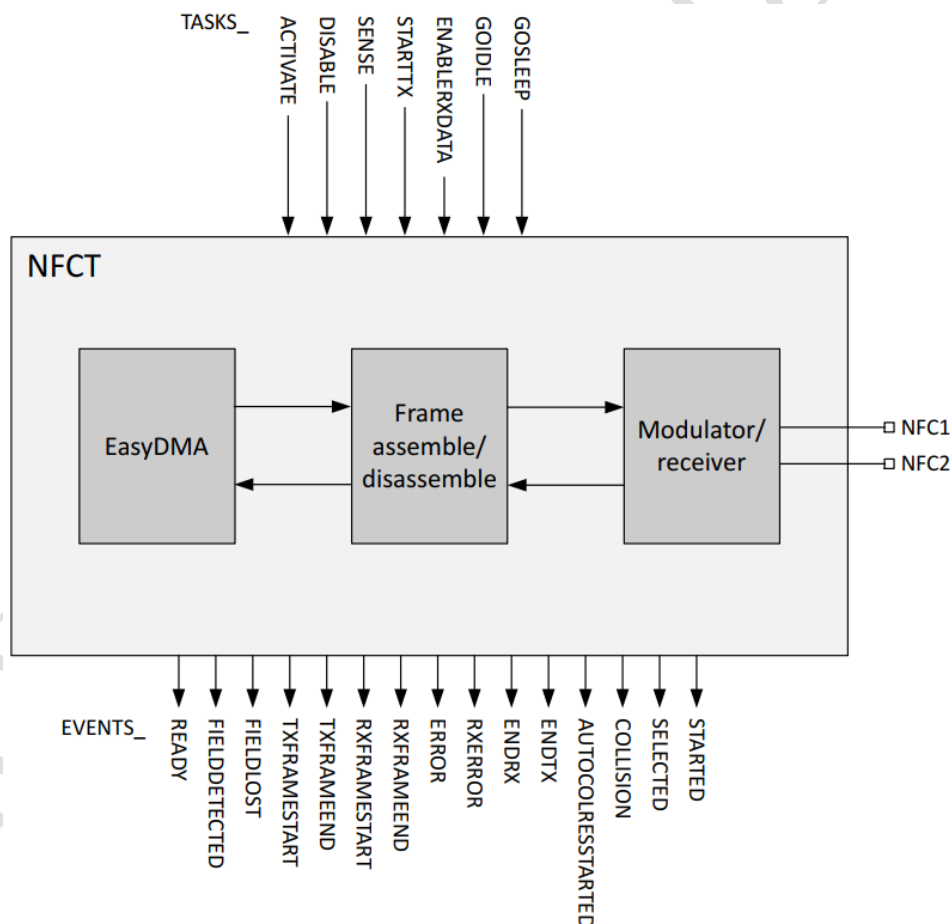
Figure 16: NFC block diagram
