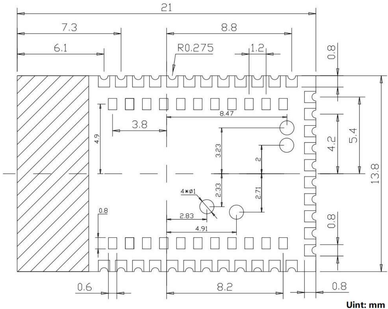
Figure 4: MK13 PCB land pads dimensions (TOP View)
