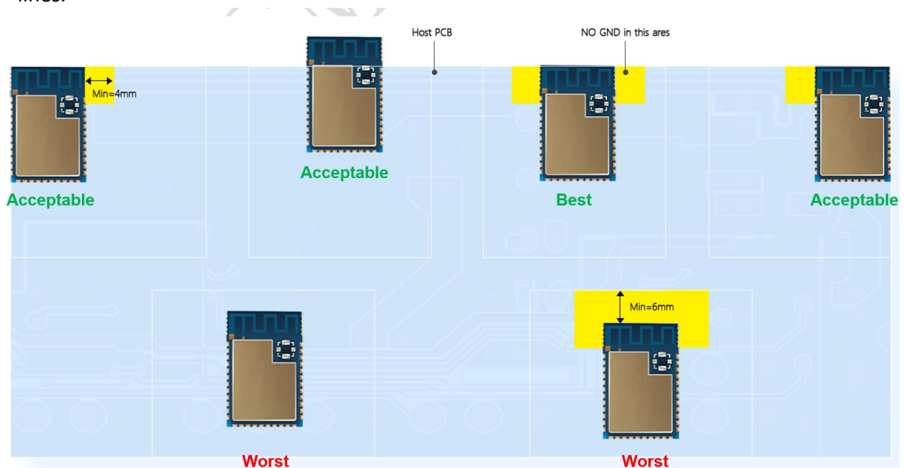
Figure 18: Recommended Module Mounting Examples
