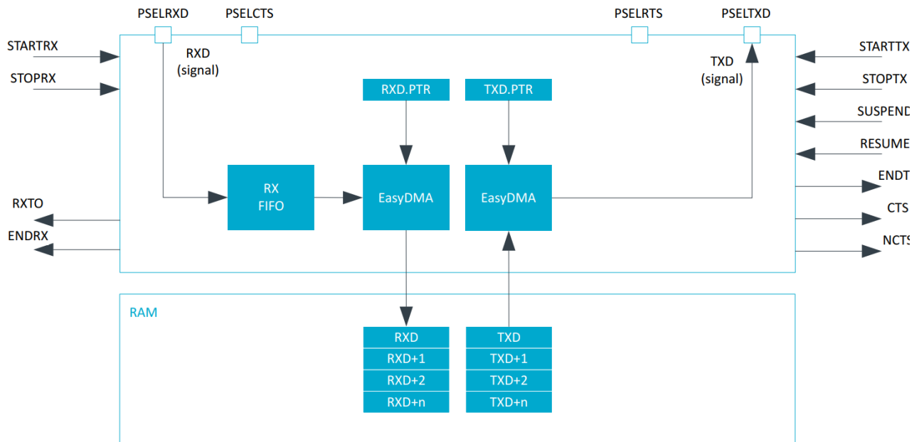
Figure 14: UART configuration
